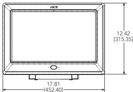
NXT-CV17 (Front)
